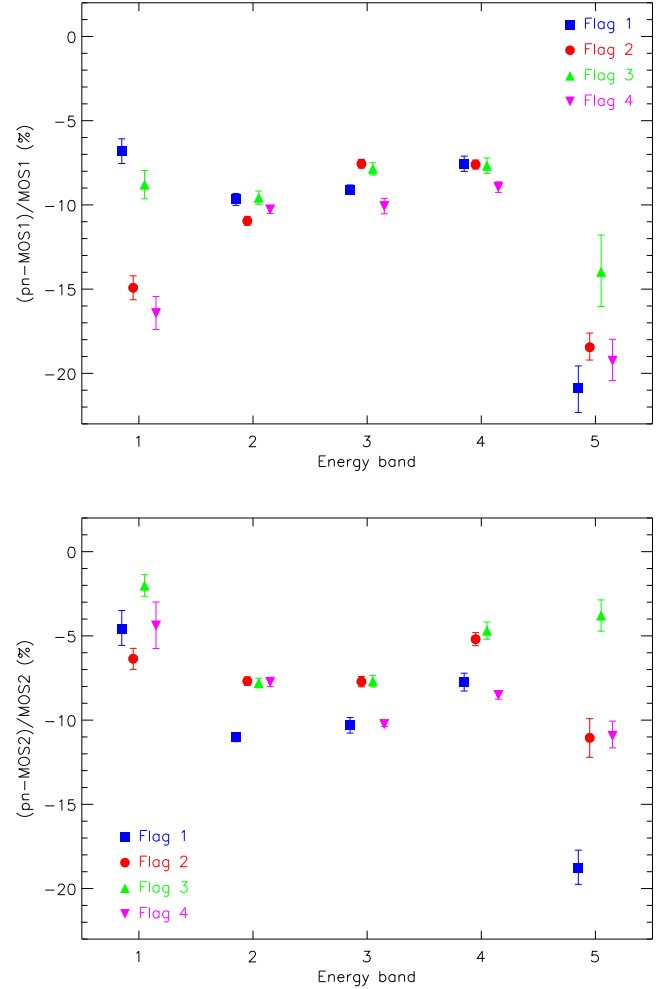
Fig. 8. Variation of the percentage flux difference between the EPIC cameras as a function of the azimuthal position of the sources in the FOV of the MOS cameras (see Sec. 4.3 and Fig. 9). Only sources with MOS off-axis values >2' have been included in the analysis. The x-axis shows the energy band identification number used in this work: 1: 0.2-0.5 keV, 2: 0.5-1.0 keV, 3: 1.0-2.0 keV, 4: 2.0-4.5 keV and 5: 4.5-12.0 keV. Data points at each energy band have been shifted slightly along the x-axis for clarity. Errors are 90% confidence.
