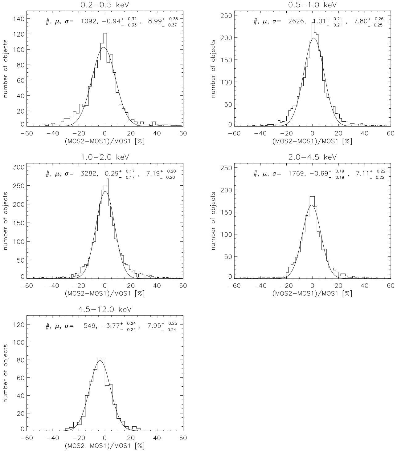
Fig. 4. Distributions of the percentage flux difference between the EPIC MOS1 and MOS2 cameras as a function of the energy band. The best-fit of the experimental distributions with a Gaussian function is shown with a smooth solid line and the corresponding best-fit parameters (mean and dispersion) and number of sources involved in the analysis are listed in the upper-left corner of the plots (also given in Table 2). Errors are 90% confidence.
