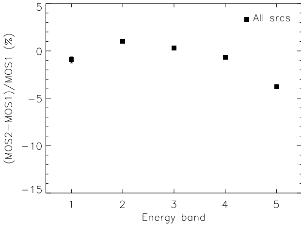
Fig. 5. Mean percentage flux difference between the EPIC cameras as a function of energy. The x-axis shows the energy band identification number used in this work: 1: 0.2-0.5 keV, 2: 0.5-1.0 keV, 3: 1.0-2.0 keV, 4: 2.0-4.5 keV and 5: 4.5-12.0 keV. Top: pn-MOS1 comparison. Middle: pn-MOS2 comparison. Bottom: MOS2-MOS1 comparison. Errors are 90% confidence.
