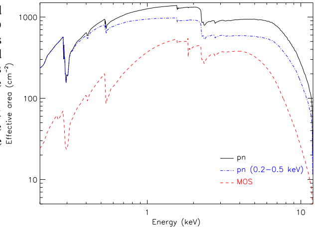
Fig. 2. Variation of the effective area of the EPIC cameras (for the medium filter) as a function of energy. The dot-dashed and solid lines show the effective area for the EPIC pn camera, for single pixel events (used below 0.5 keV) and for single+double pixel events (used above 0.5 keV) respectively. The dashed line shows the effective area for the EPIC MOS cameras.
