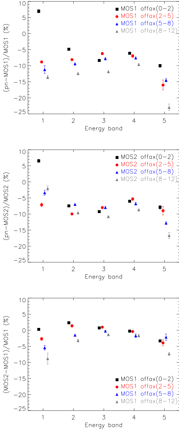
Fig. 7. Variation of the percentage flux difference between the EPIC cameras as a function of the energy band for sources at different MOS off-axis angles. The x-axis shows the energy band identification number used in this work: 1: 0.2-0.5 keV, 2: 0.5-1.0 keV, 3: 1.0-2.0 keV, 4: 2.0-4.5 keV and 5: 4.5-12.0 keV. Data points at each energy band have been shifted slightly along the x-axis for clarity. Top: pn-MOS1 comparison. Middle: pn-MOS2 comparison. Bottom: MOS2-MOS1 comparison. Errors are 90% confidence.
