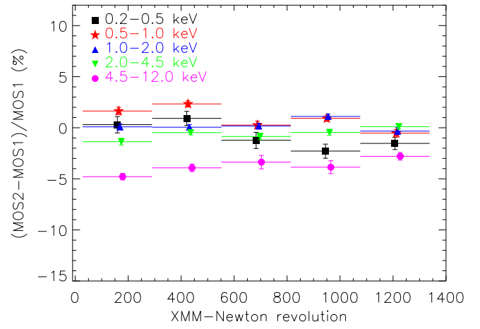
Fig. 6. Percentage flux difference between the EPIC cameras at different energies as a function of time. Top: pn-MOS1 comparison. Middle: pn-MOS2 comparison. Bottom: MOS2-MOS1 comparison. Errors are 90% confidence.
