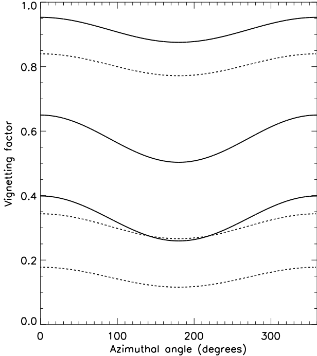
Fig. 10. MOS vignetting factor as a function of azimuthal angle at energies of 1 keV (solid lines) and 10 keV (dotted lines), and for off-axis angles of (top to bottom) 3', 9' and 15'.
