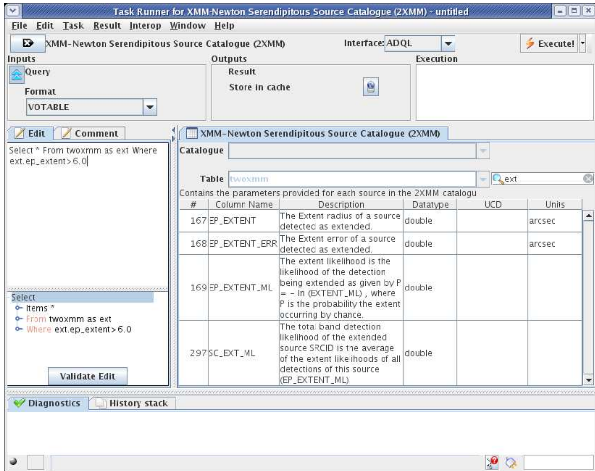
Figure 4. Advanced querying including pre-filtering on catalogue parameters: select an ADQL query interface to a 2XMMi X-ray catalogue resource using VOExplorer, then identify columns in the catalogue corresponding to “extent”. The user may then construct a simple but powerful query against these parameters in the “Edit” pane using a standard “ADQL” query language and here extract all extended sources (which the user has defined as having extent radius greater than 6.0 arcseconds) to create a new science sample in VOTable format for further visualisation and analysis.
